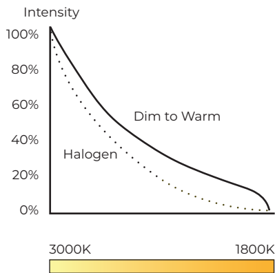
Dim to Warm dimming curve compared to halogendimming curve compared to halogen
